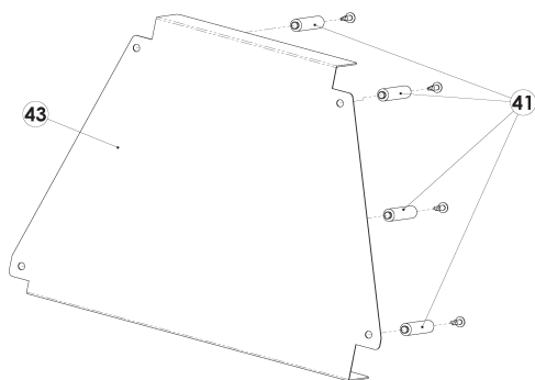
Detail F
