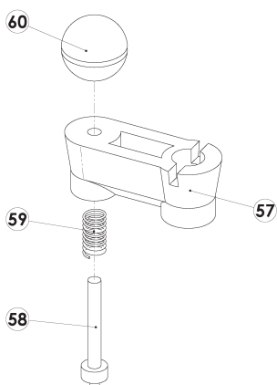
Detail G
