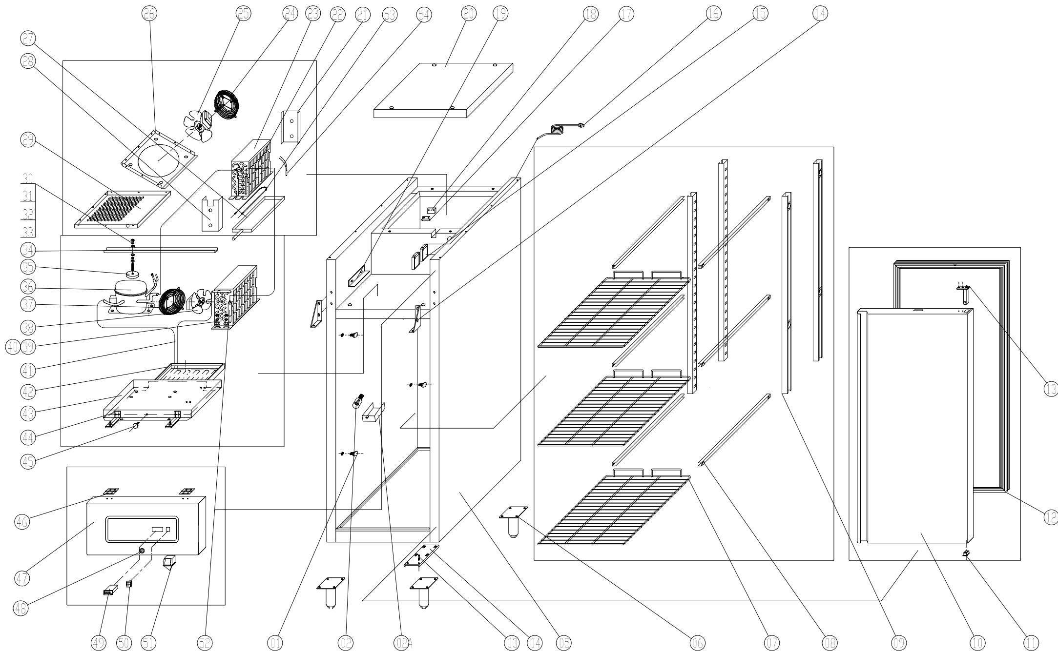
EXPLODE DIAGRAM OF GN650TN(WITH H.E.)
