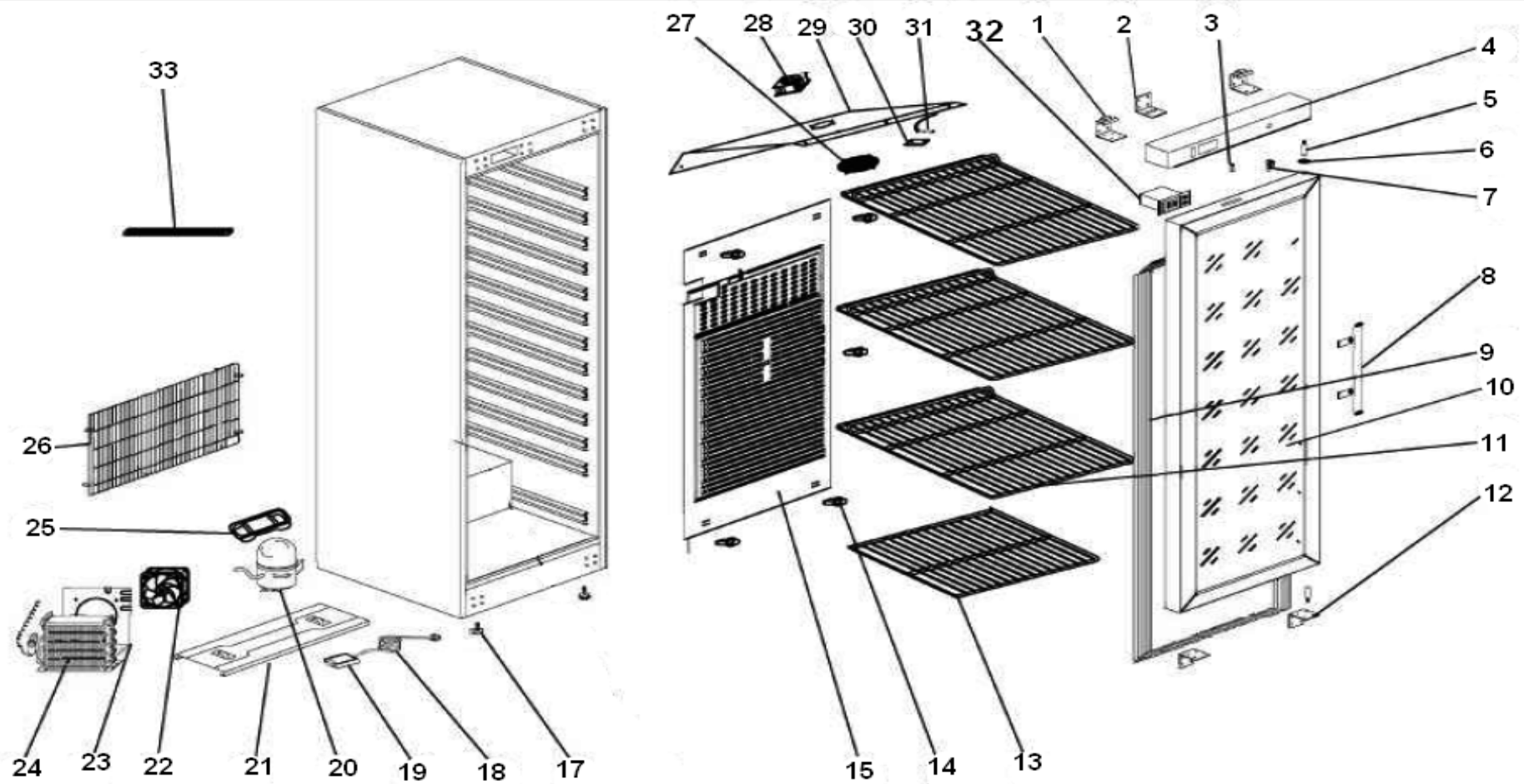
EXPLODE OF ER/ ERG/EF400 ER/ EF 400SS
