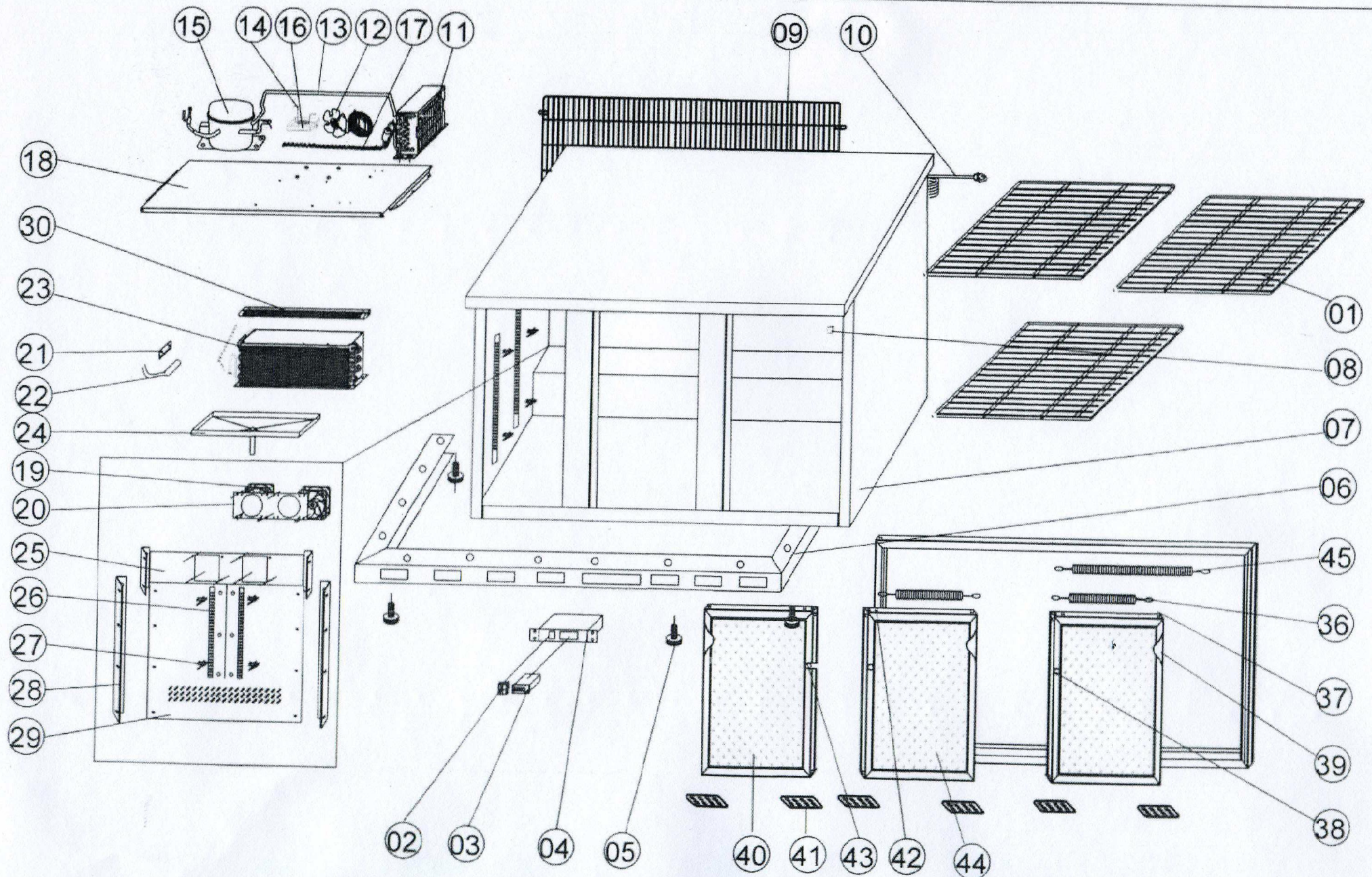
EXPLODE DRAWING OF BC3PS
