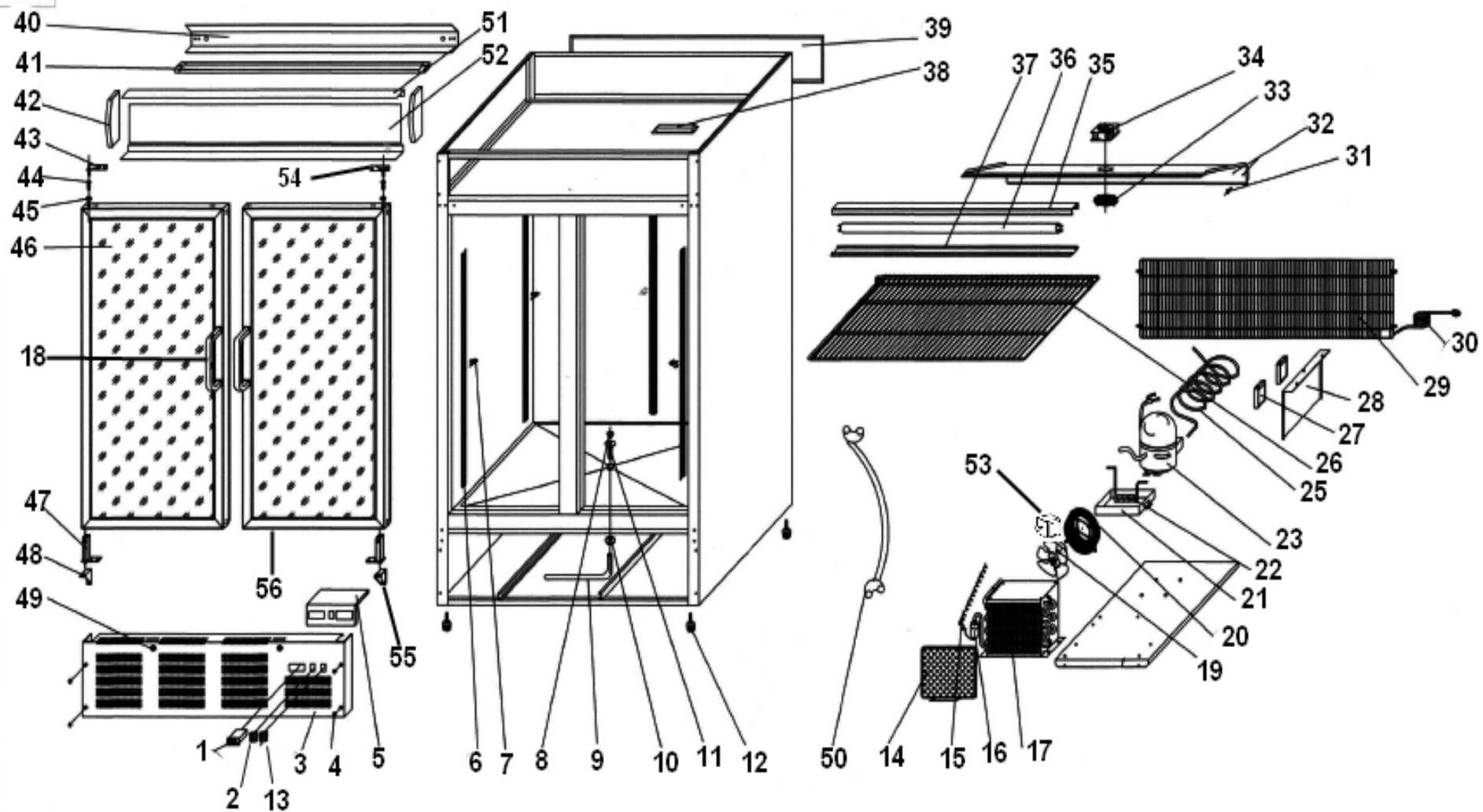
EXPLODE OF SNACK 638-340 TNG
