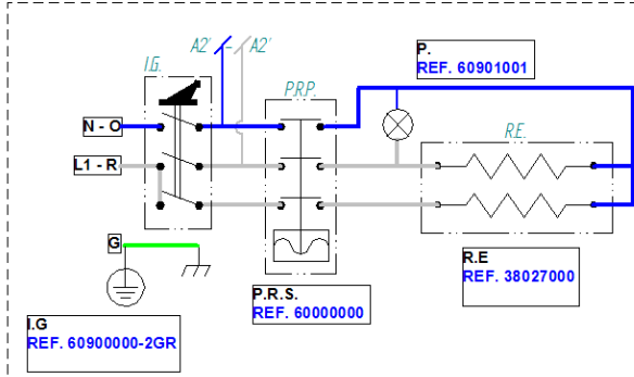
(OPTIONAL) 230V 1N~ HEATING ELEMENT 3050W - 2GR
