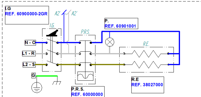
(OPTIONAL) 230V 1N~ HEATING ELEMENT 3050W - 2GR
