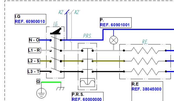
(OPTIONAL POWERED) 400V 3N~ HEATING ELEMENT 4500W - 2G
