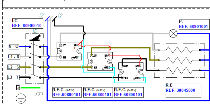
(OPTIONAL POWERED) 400V 3N~ HEATING ELEMENT 4500W - 2GR
