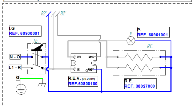
(STANDARD) 230V 1N~ HEATING ELEMENT 3050W- 2GR
