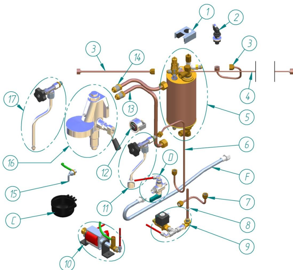
EXPLODED VIEW OFFICE LEVA WATER NETWORK CONNECTION
